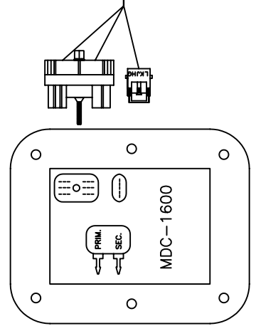
PLUG CONNECTORS ONTO MDC-1600
